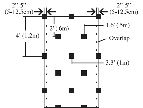
C 1.7 staples per square yard (2 staples per square metre)
